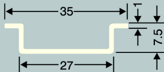
DNR - 35U Mounting Rail 7.5 x 35 x 1 mm
