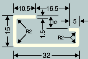
DNR - 32G Mounting Rail 'G' Type 32 x 15 x 1.5 mm
