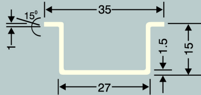
DNR - 35D 'U' Rail 15 x 35 x 1.5 mm
